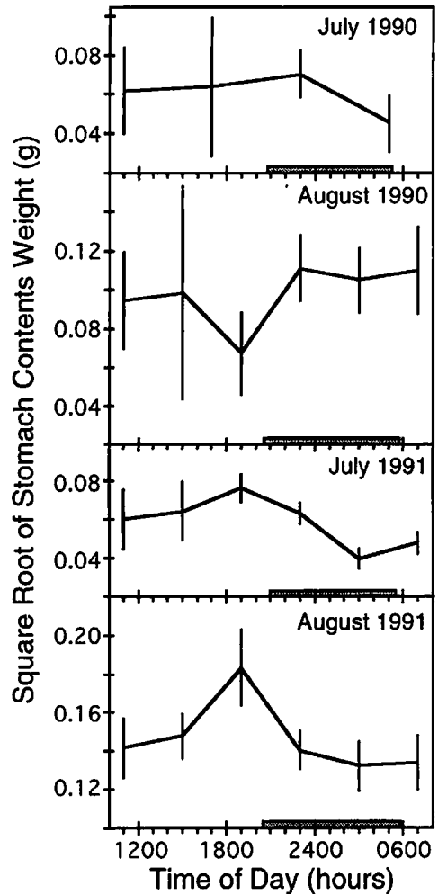
FIGURE 8.—Diel periodicity of weight of stomach contents for age-0 ruffes on four collection dates. For each time period, a least-squares mean and Bonferroni-corrected 95% confidence interval (vertical bar) was estimated with an ANCOVA model with time period as a factor and body weight as a covariate. The shaded bar on each abscissa indicates the period between sunset and sunrise. Each ordinate has the same scale but a different range.
